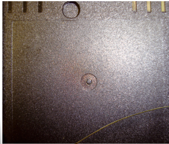
Figure 1 Evidence of an anti-wear insert around a small valve pin gate
